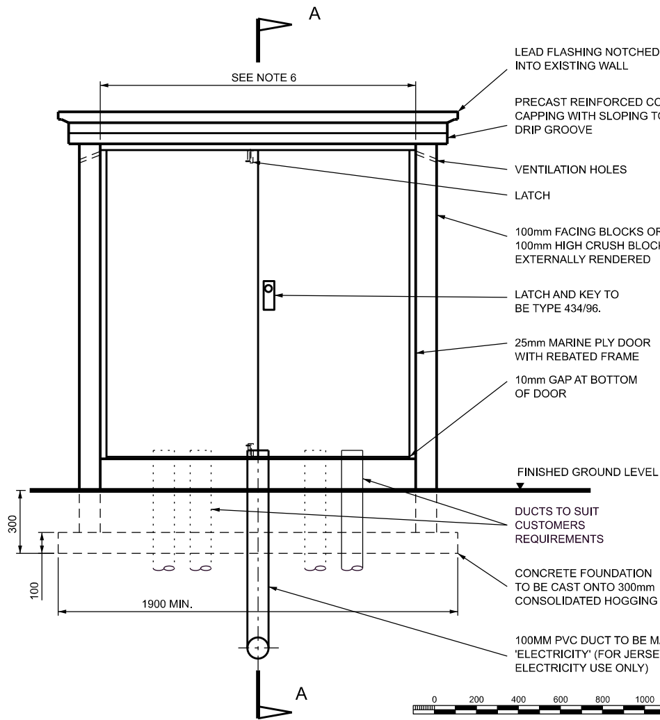
FRONT ELEVATION
